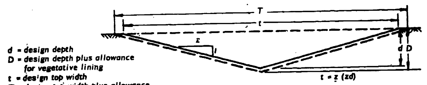
TRIANGULAR CROSS SECTION
