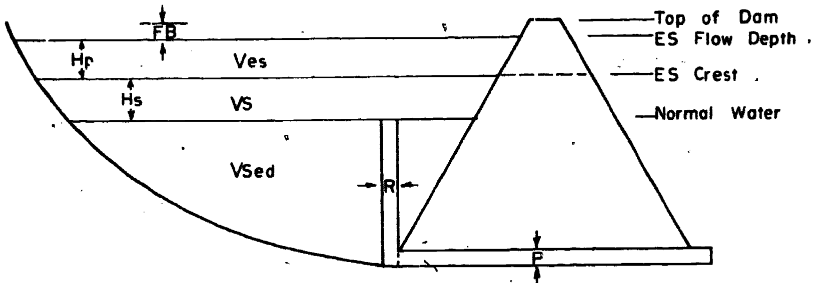
Profile Thru Dam
