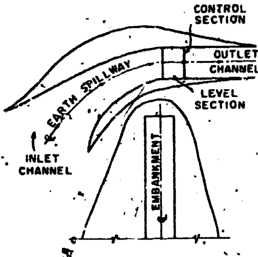
PLAN OF EARTH SPILLWAY
