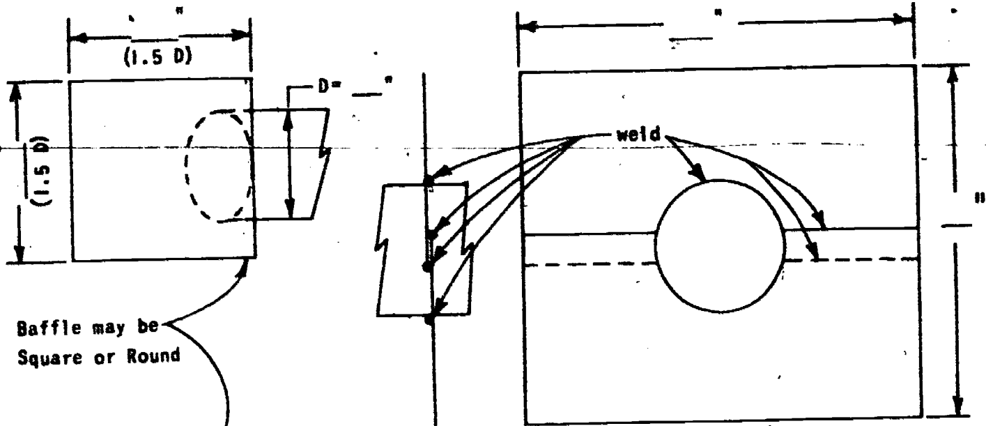
ANTI-SEEP COLLAR
