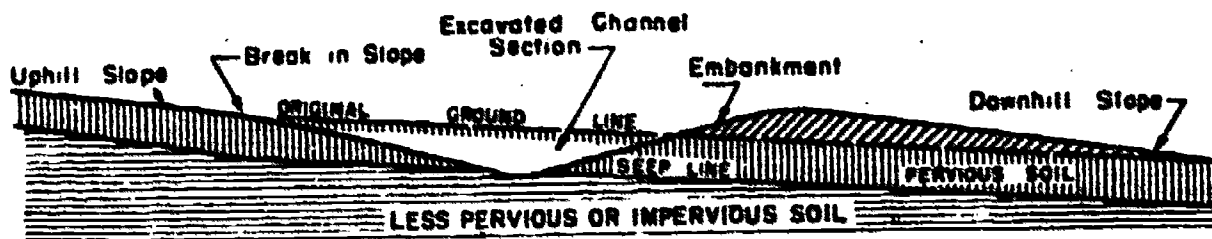
A. - CROSS SECTION SHOWING DITCH AS SURFACE WATER DIVERSION AND SUB-SURFACE INTERCEPTOR ON SLOPE
