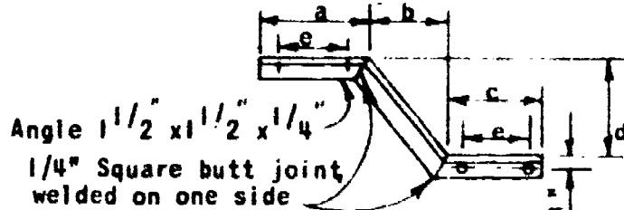
ANGLE BRACE DETAIL
