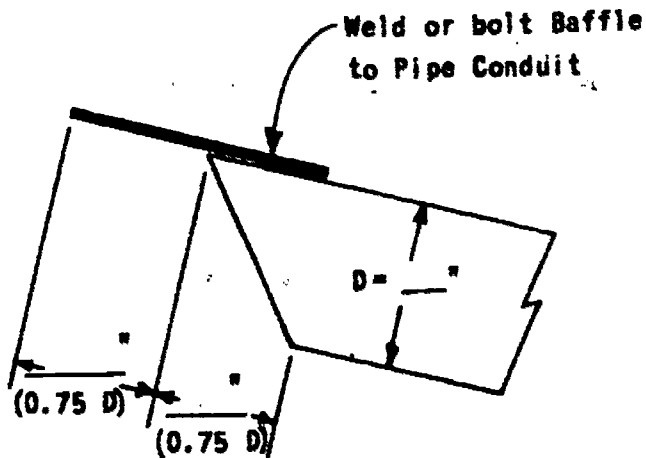
INLET SECTION
