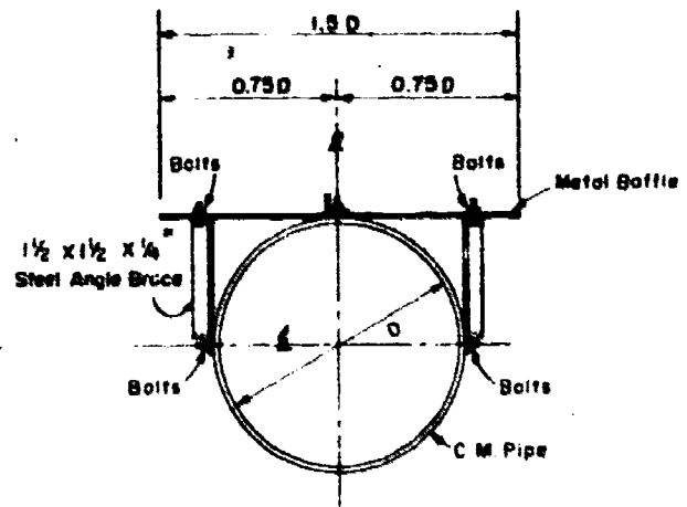
FRONT ELEVATION
