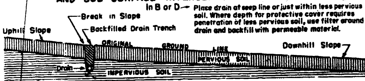
D. - CROSS SECTION SHOWING DRAIN AS SUB-SURFACE INTERCEPTOR
