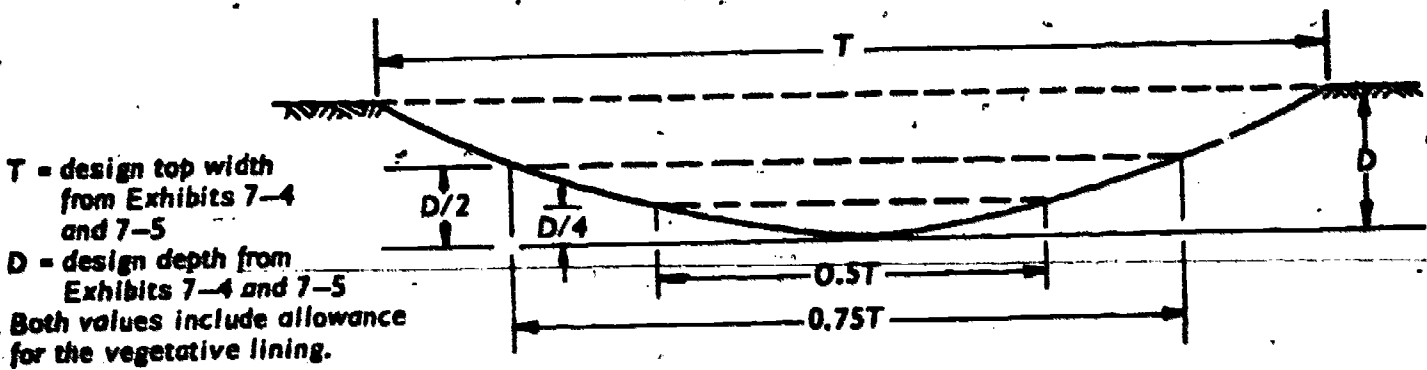
PARABOLIC CROSS SECTION
