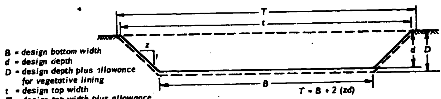
TRAPEZOIDAL CROSS SECTION
