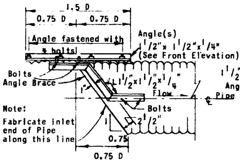
SIDE ELEVATION
