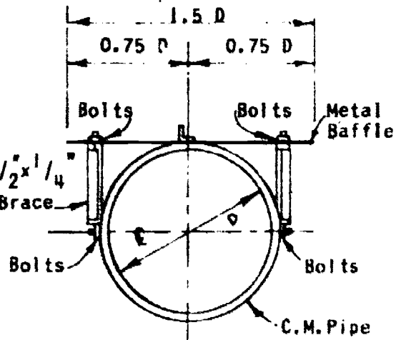
ANGLE BRACE DETAIL
