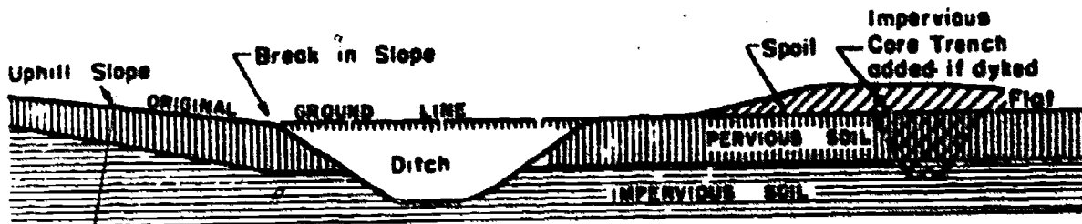
C. - CROSS SECTION SHOWING DITCH AS SURFACE WATER DIVERSION AND SUB-SURFACE INTERCEPTOR FOR FLAT LAND
